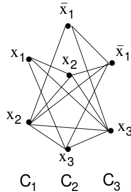
Figure 17.6 The graph generated from Boolean expression B = (x_1 + x_2) \cdot (\bar{x}_1 + x_2 + x_3) \cdot (\bar{x}_1 + x_3) . Literals from the first clause are labeled C1, and literals from the second clause are labeled C2. There is an edge between every pair of vertices except when both vertices represent instances of literals from the same clause, or a negation of the same variable. Thus, the vertex labeled C1 : y_1 does not connect to the vertex labeled C1 : y_2 (because they are literals in the same clause) or the vertex labeled C2 : \bar{y}_1 (because they are opposite values for the same variable).
