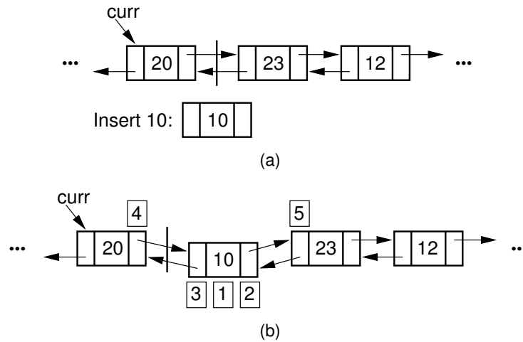
Figure 4.15 Insertion for doubly linked lists. The labels 1 , 2 , and 3 correspond to assignments done by the linked list node constructor. 4 marks the assignment to curr -> next . 5 marks the assignment to the prev pointer of the node following the newly inserted node.
